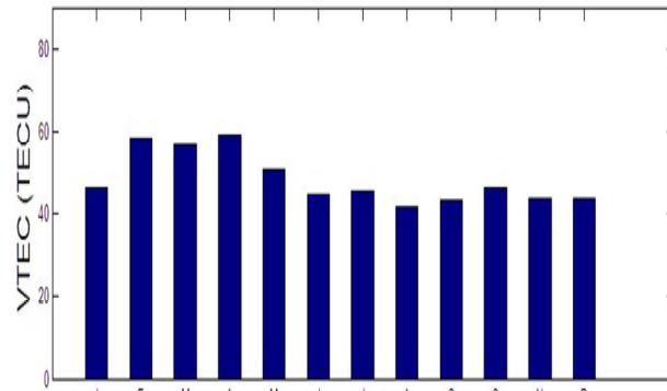
Fig. 2. 2007 Monthly variations of VTEC
