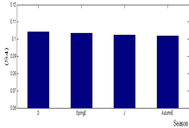
Fig. 13. 2009 Seasonal variation of S4
