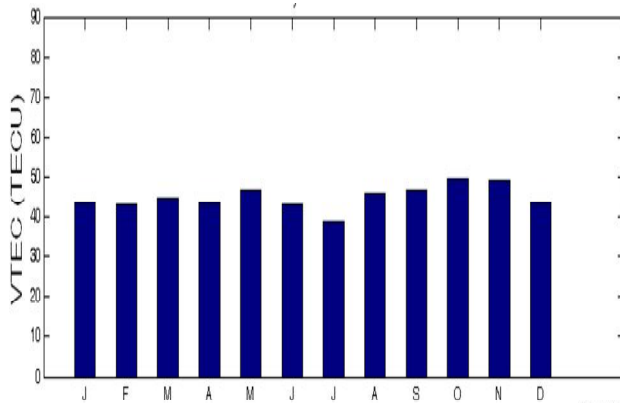
Fig. 4. 2009 Monthly variation of VTEC
