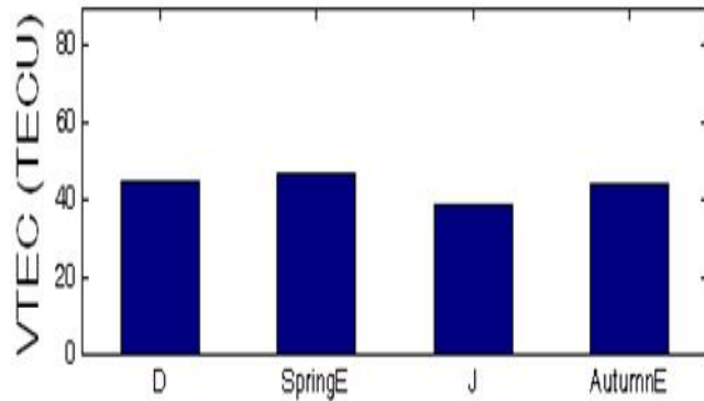
Fig. 6. 2008 Seasonal variations of VTEC Season
