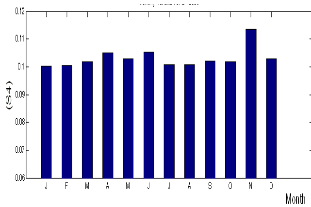
Fig. 10. 2009 Monthly variation of S4
