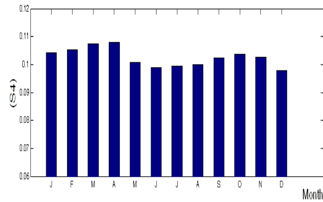
Fig. 9. 2008 Monthly variation of S4
