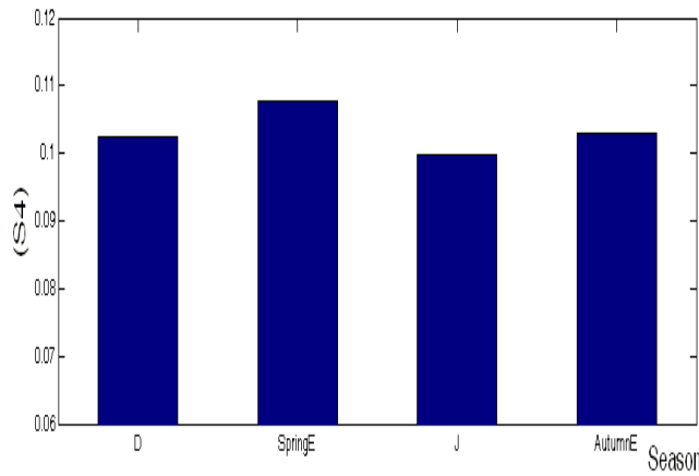
Fig. 12. 2008 Seasonal variation of S4
