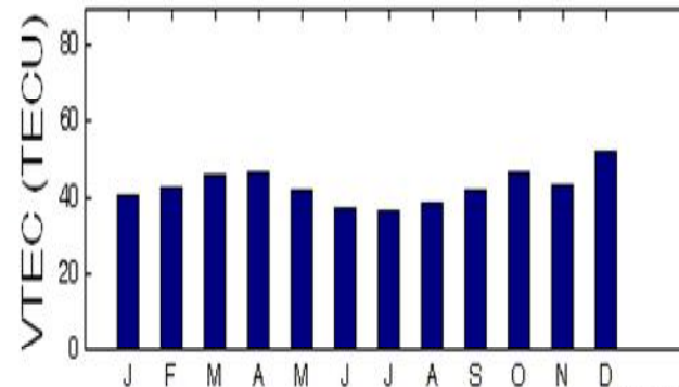
Fig. 3. 2008 Monthly variations of VTEC
