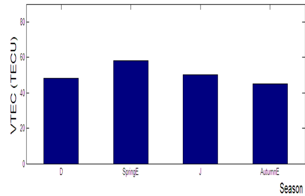
Fig. 5. 2007 Seasonal variations of VTEC
