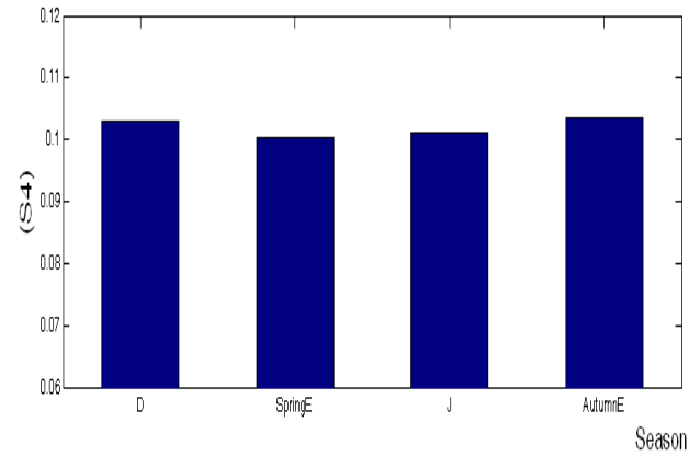
Fig. 11. 2007 Seasonal variation of S4
