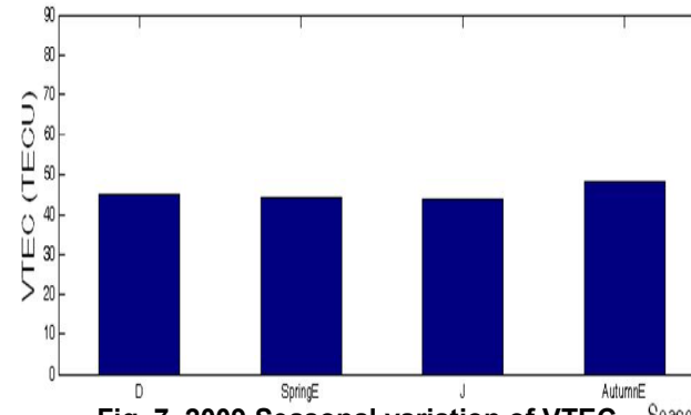
Fig. 7. 2009 Seasonal variation of VTEC Season
