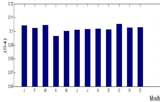
Fig. 8. 2007 Monthly variations of S4
