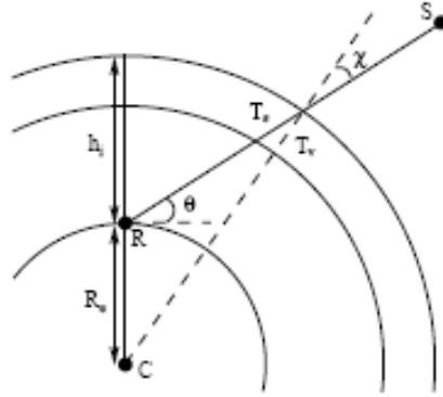
Fig. 1. Geometry of a GPS satellite-receiver link
