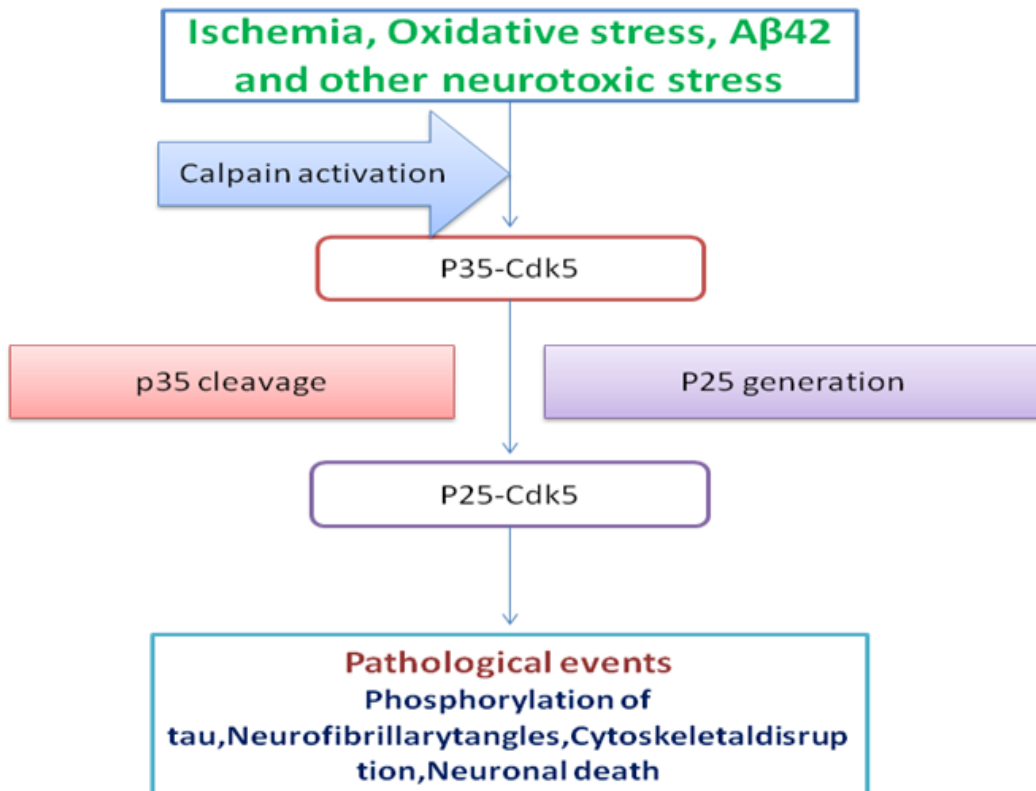
Fig. 2. The deregulation of CDK5 activity
