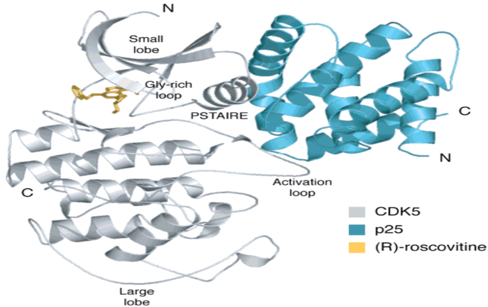
Fig. 1. Ribbon diagram of the CDK5/p25 complex
