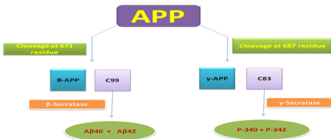
Fig. 3. Processing of Amyloid precursor protein
